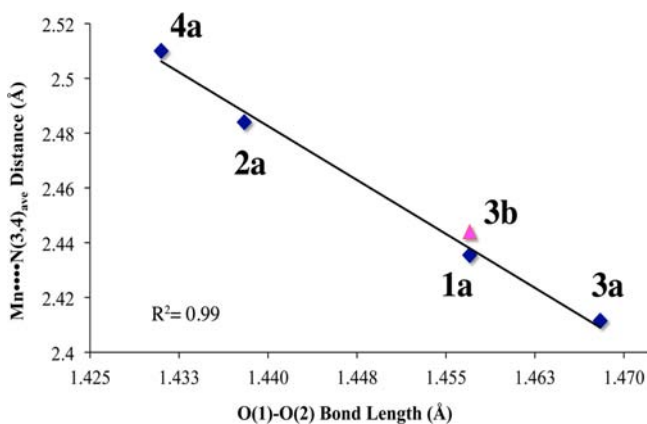
Figure 4. Plot of O(1)–O(2) bond length (Å) vs Mn(III)–N(3,4) avg distance (Å) for Et-linked ( 1a , 3b , and 3a ), and Pr-linked ( 2a and 4a ) structures. Data for [\text{Mn}^{\text{III}}(\text{S}^{\text{Me}_2}\text{N}_4(6\text{-Me-DPEN}))(\text{OOCm})](\text{BPh}_4) ( 3b ) is represented by the pink triangle and is not included in the linear fit correlation coefficient ( R^2 ).
