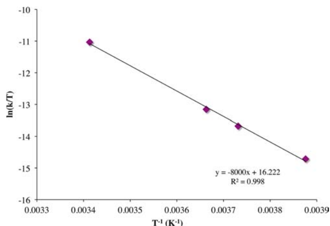
Figure 8. Eyring plot from the variable-temperature decay kinetics data for [\text{Mn}^{\text{III}}(\text{S}^{\text{Me}_2}\text{N}_4(6\text{-Me-DPPN}))(\text{OO}^t\text{Bu})](\text{BPh}_4) ( 4a ) in \text{CH}_2\text{Cl}_2 .
