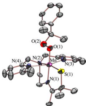
Figure 9. ORTEP diagram (50% probability ellipsoids) of [\text{Mn}^{\text{III}}(\text{S}^{\text{Me}_2}\text{N}_4(6\text{-Me-DPEN}))(\text{OOCm})]^+ ( 3b ) showing exceptionally long \text{Mn}\cdots\text{N}(3,4) intermolecular interactions as dashed lines. Hydrogen atoms, counterions, and solvent of crystallization have been omitted for clarity.
