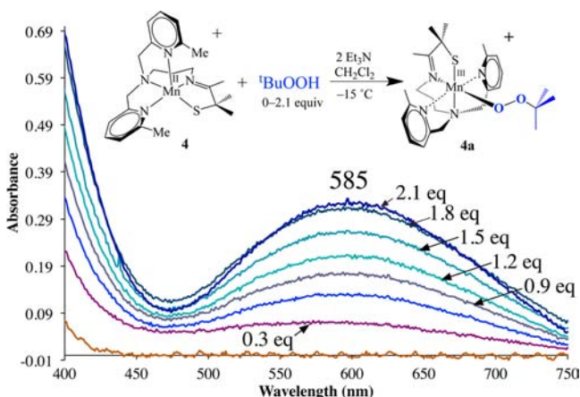
Figure 1. Titration of 0–2.1 equiv of t BuOOH (in 0.3-equiv aliquots) to a CH 2 Cl 2 solution [Mn II (S Me 2 N 4 (6-Me-DPPN)](BPh 4 ) (4; 2.2 mM), in the presence of 2 equiv of Et 3 N, at –15 °C as monitored by visible absorption spectroscopy.
